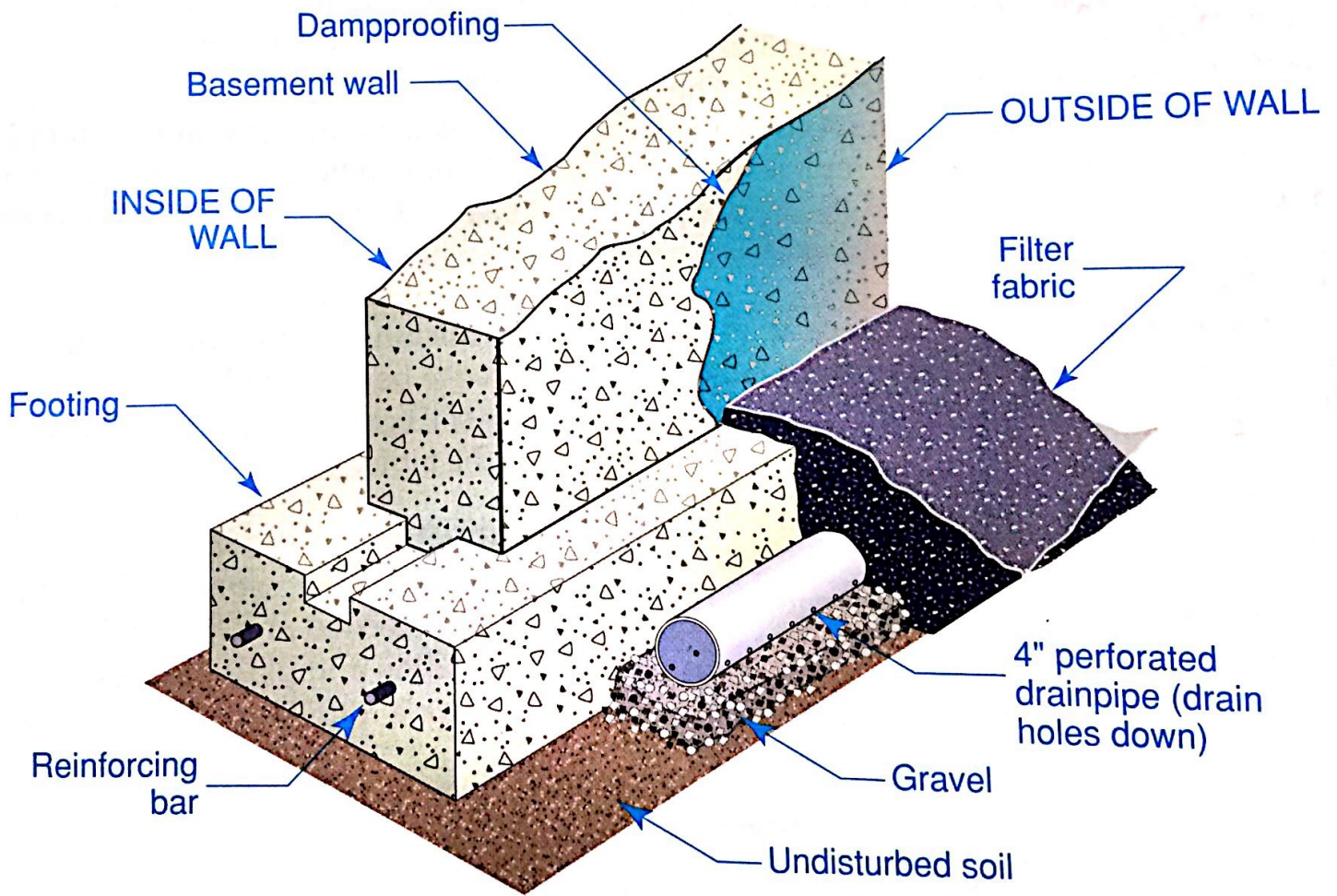
Figure 10-6 Foundation Drains Pressure Relief Footing drains prevent water from building up against foundation walls.
